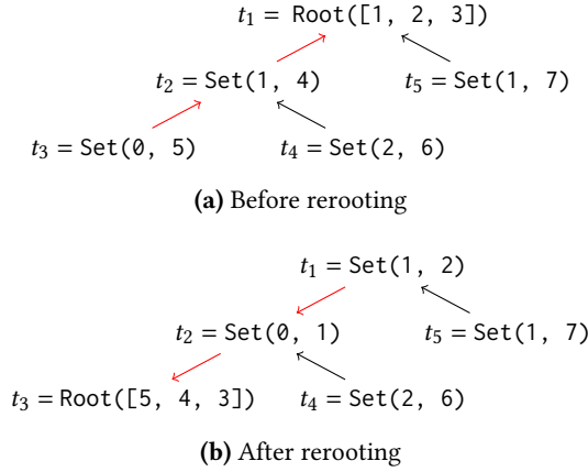
Figure 2. Rerooting of node t_3 in a tree of persistent arrays.
